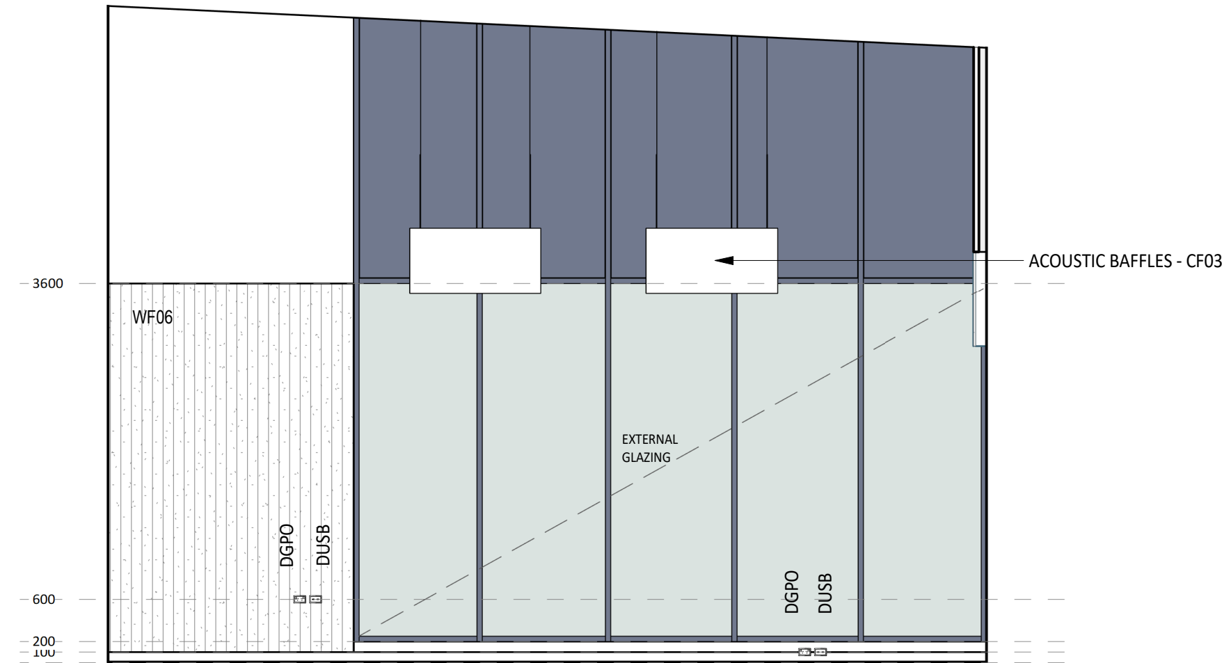
5 ELEVATION DETAIL 60-048 1 : 50
