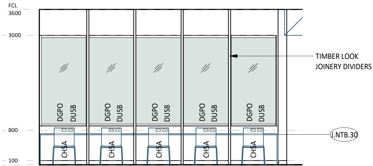
4 ELEVATION DETAIL 60-048 1 : 50
