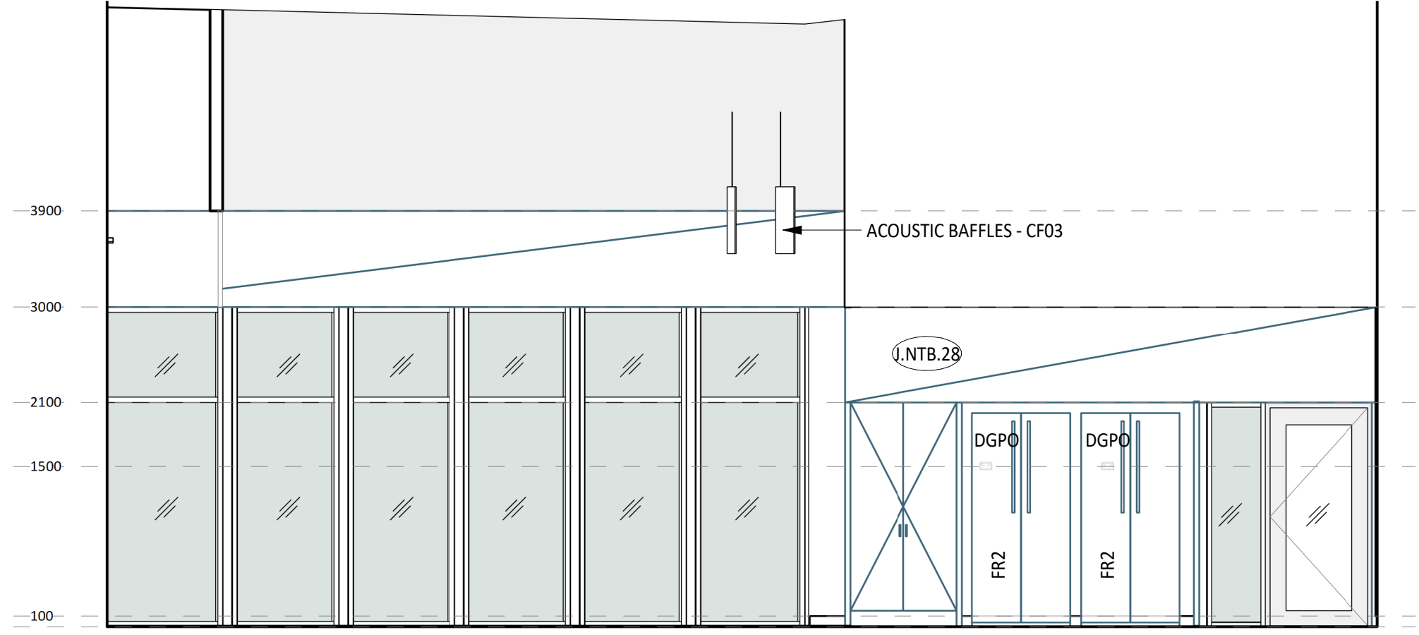
2 ELEVATION DETAIL 60-048 1 : 50
