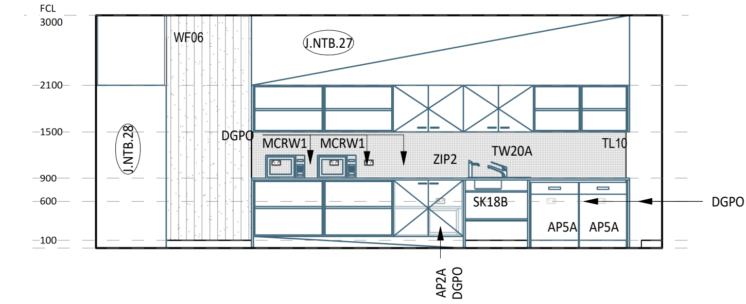
3 ELEVATION DETAIL 60-048 1 : 50
